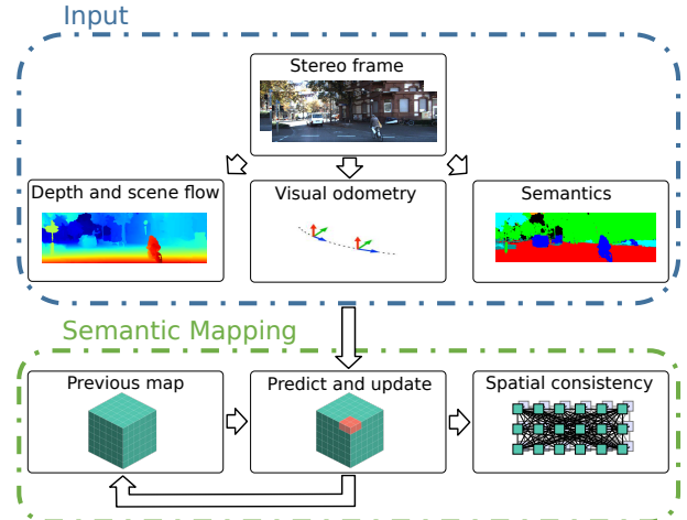
Fig. 1. We map dynamic environments in 3D occupancy grid maps using stereo visual odometry, depth, and scene flow. Image-based semantic segmentation is additionally temporally filtered in the semantic maps and made spatially consistent in a dense CRF. Scene motion is compensated for by warping the mapped dynamic objects with the estimated scene flow.
